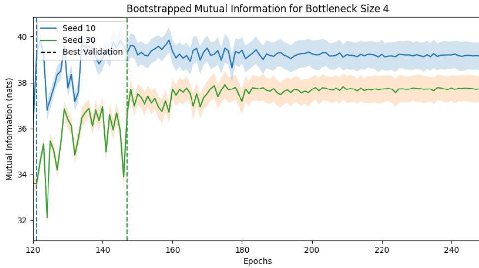
Figure 6: Mutual Information per Epoch for Bottleneck Dimension 4
