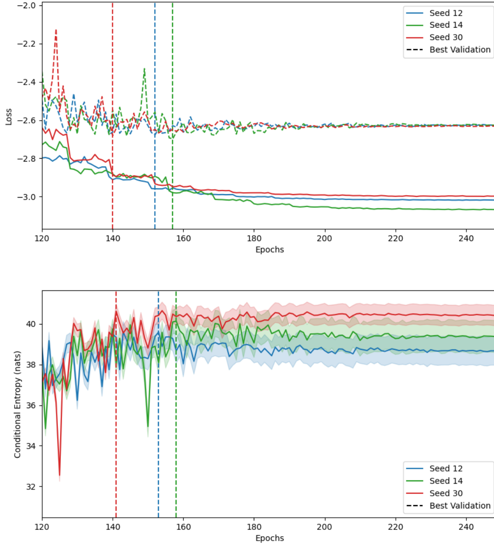
Figure 4: Conditional Entropy per Epoch for N_B = 15
