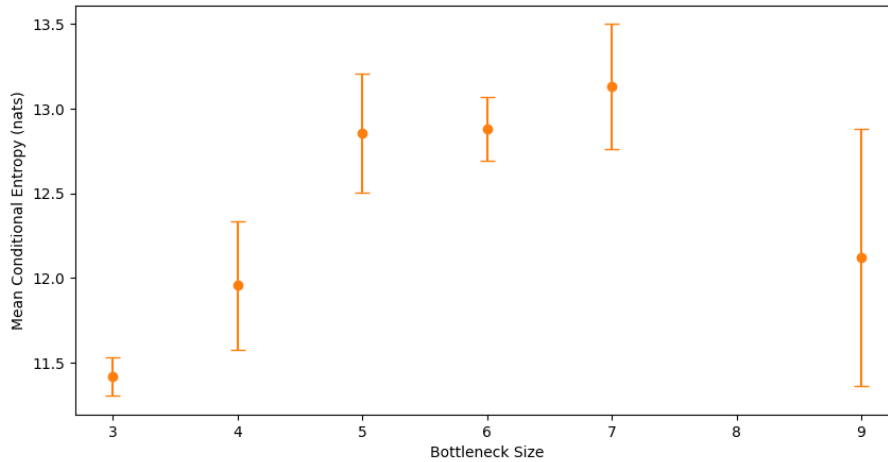
Figure 12: Final MI estimates for simulation parameter inference, 5% rule
