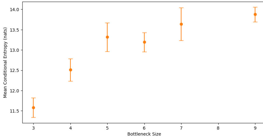
Figure 13: Final MI estimates for simulation parameter inference, best validation rule
