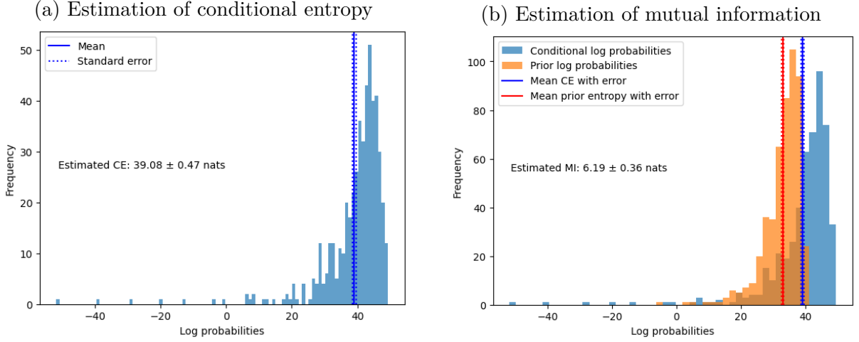
Figure 4: Histogram plots used to evaluate CE and MI
