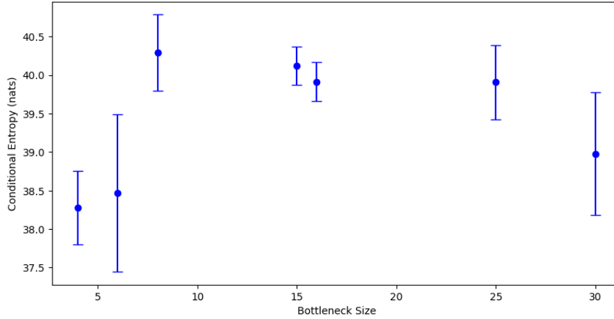
Figure 8: Final CE estimates for x_{\text{HI}} inference, last epoch rule
