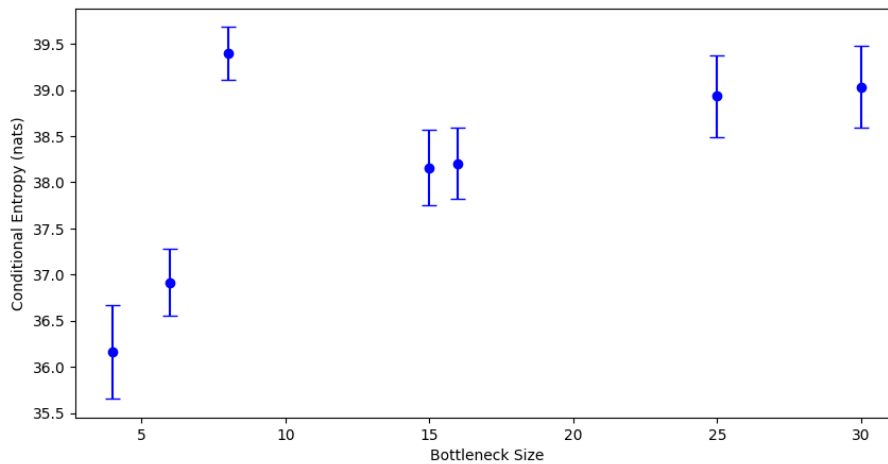
Figure 6: Final CE estimates for x_{\text{HI}} inference, 5% rule
