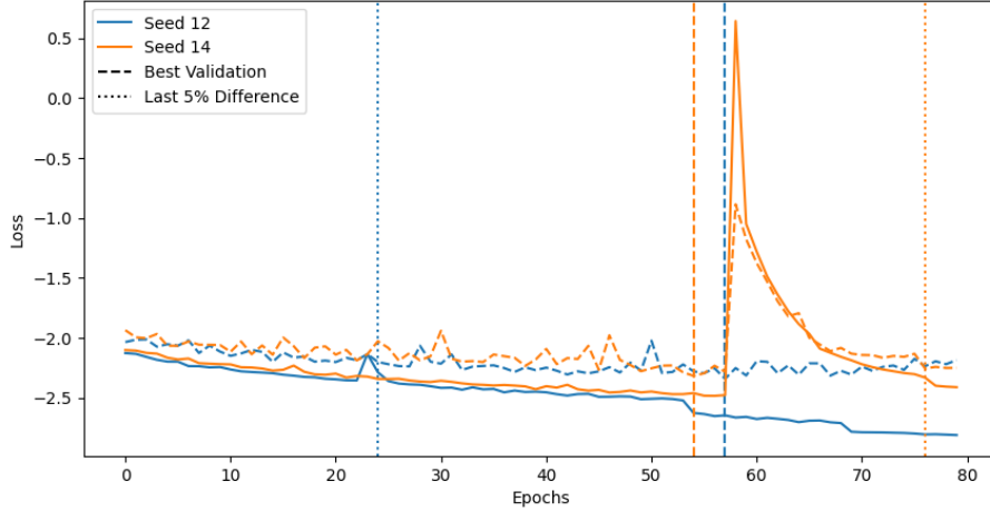
Figure 10: Model selection in finetuning for N_B = 7
