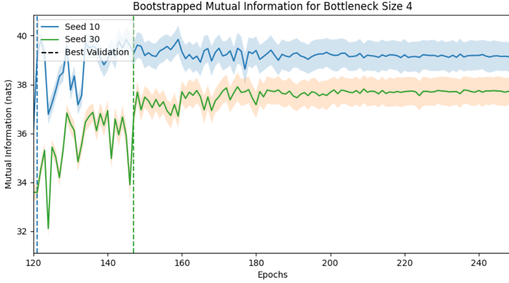
Figure 6: Mutual Information per Epoch for Bottleneck Dimension 4
