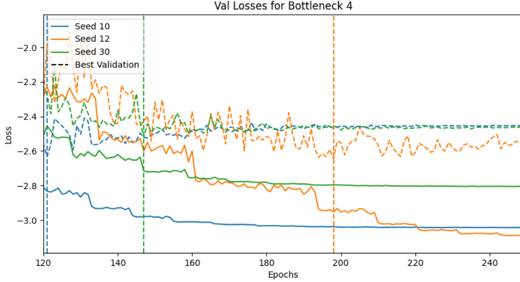
Figure 2: Train and Validation Losses for Bottleneck Dimension 4
