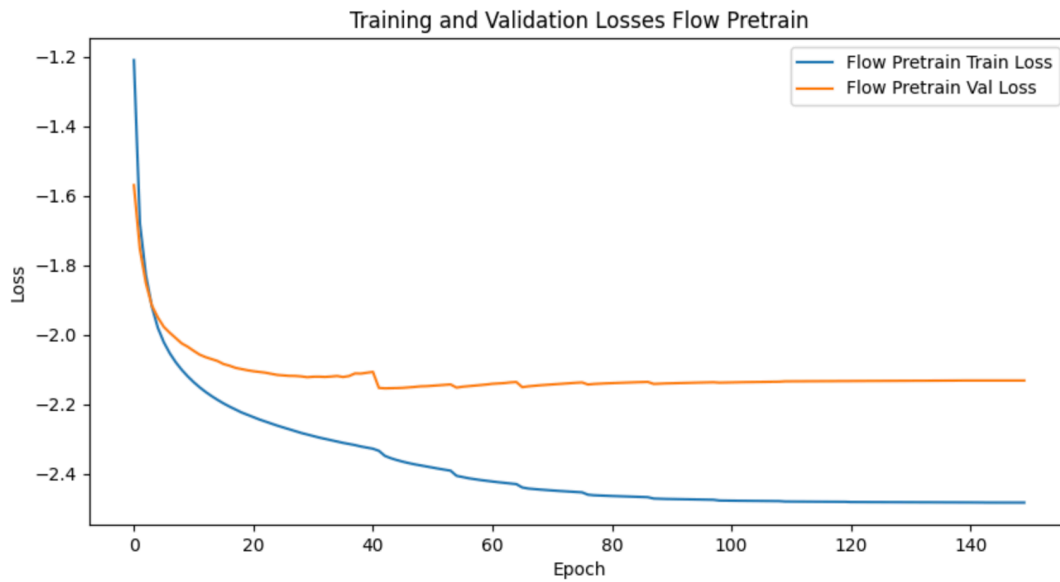
Figure 11: \mathcal{L}_{\text{NPE}} Loss Pretraining Flow
