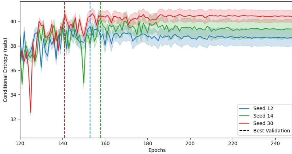
Figure 4: Conditional Entropy per Epoch for Bottleneck Dimension 15
