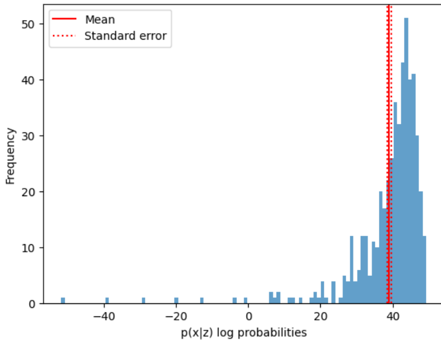
Figure 5: Histogram plot of conditional probabilities
