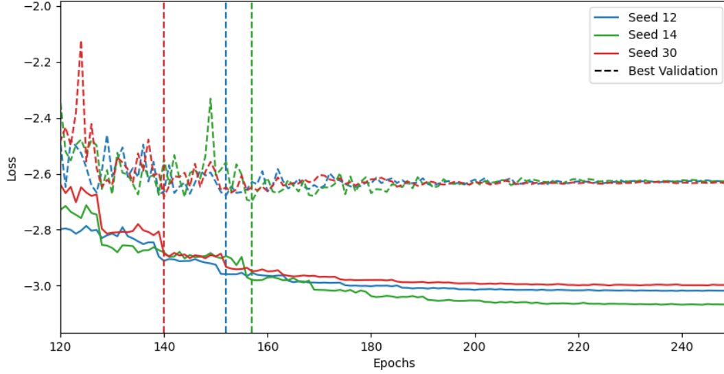
Figure 3: Train and Validation Losses for Bottleneck Dimension 15
