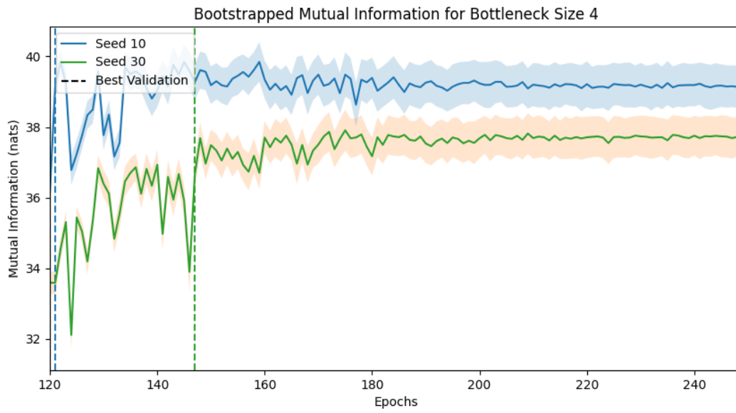
Figure 7: Mutual Information per Epoch for Bottleneck Dimension 4
