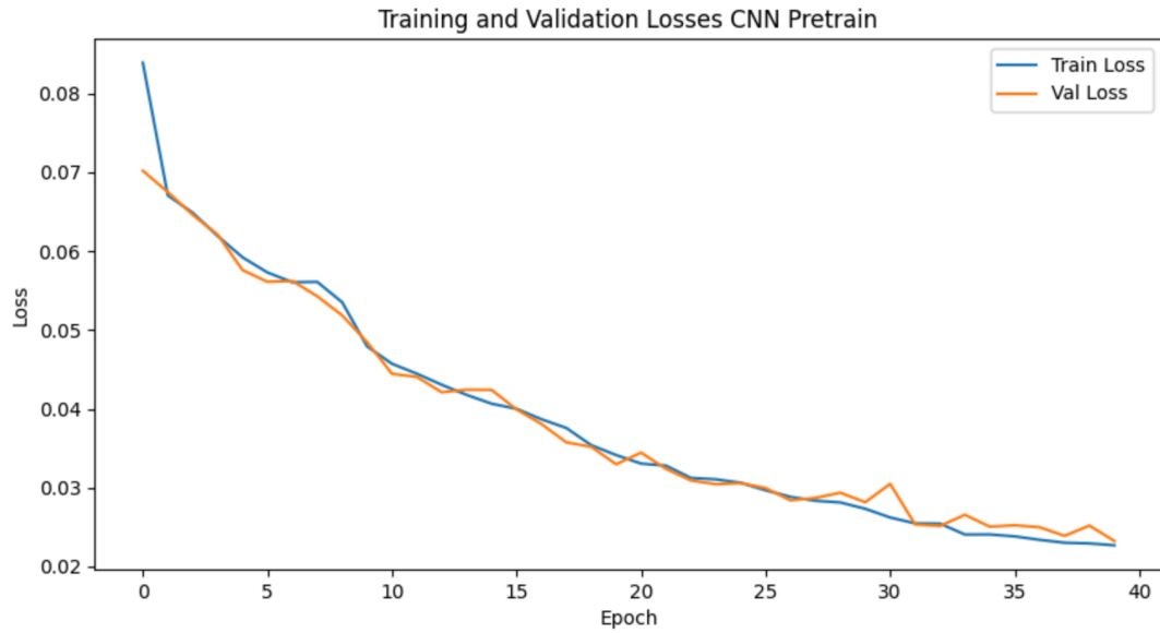
Figure 11: MSE Pretraining Loss CNN
