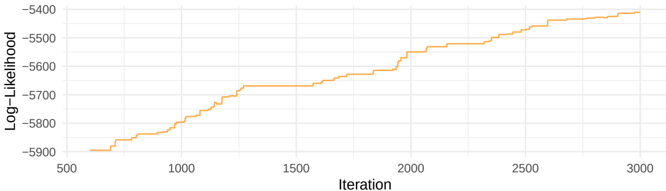
Trace Plot of Log-Likelihood
