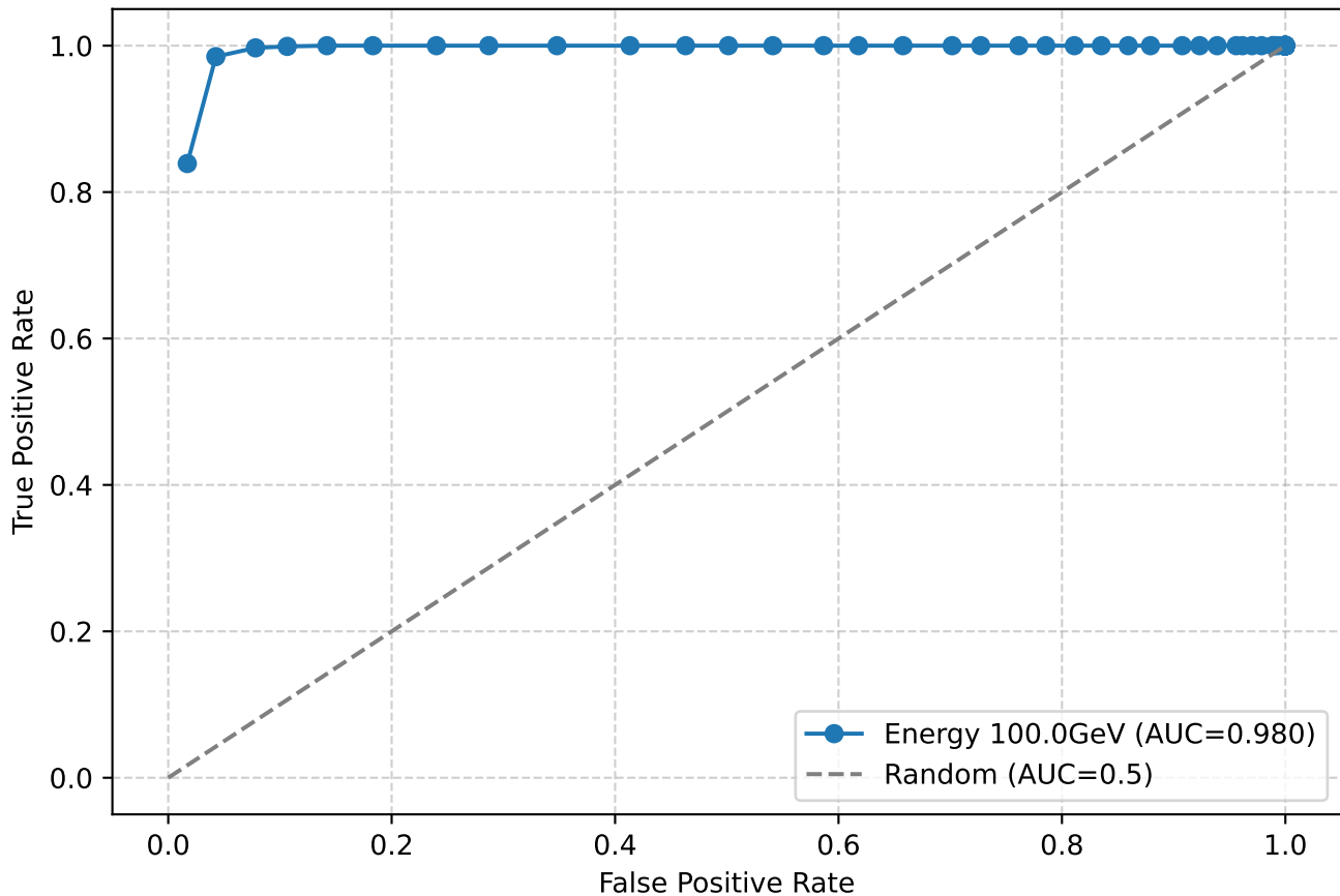
ROC Curve for electrons at 100.0GeV
