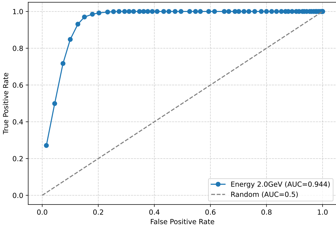
ROC Curve for electrons at 2.0GeV
