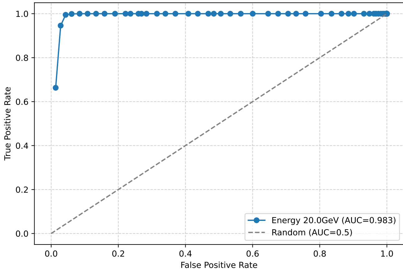
ROC Curve for electrons at 20.0GeV
