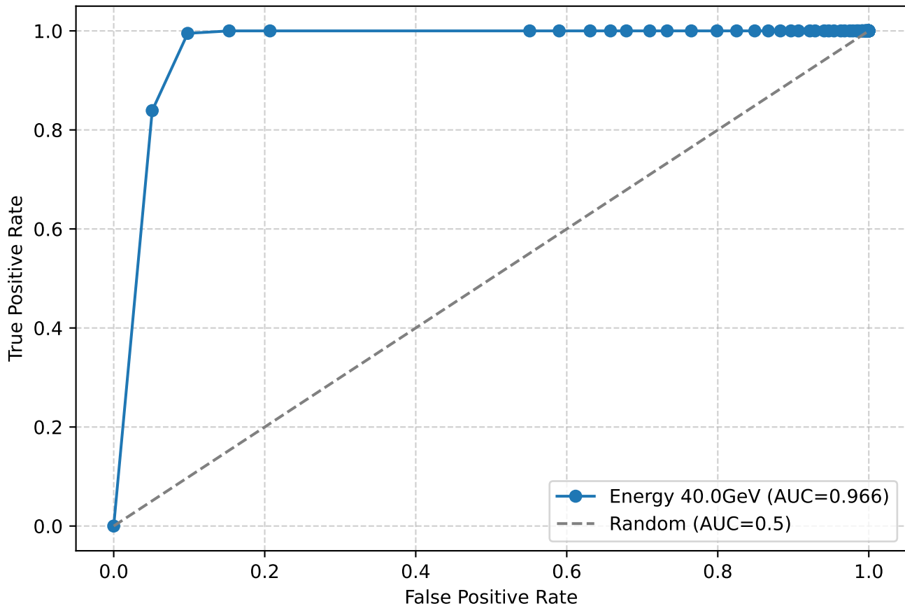
ROC Curve for electrons at 40.0GeV
