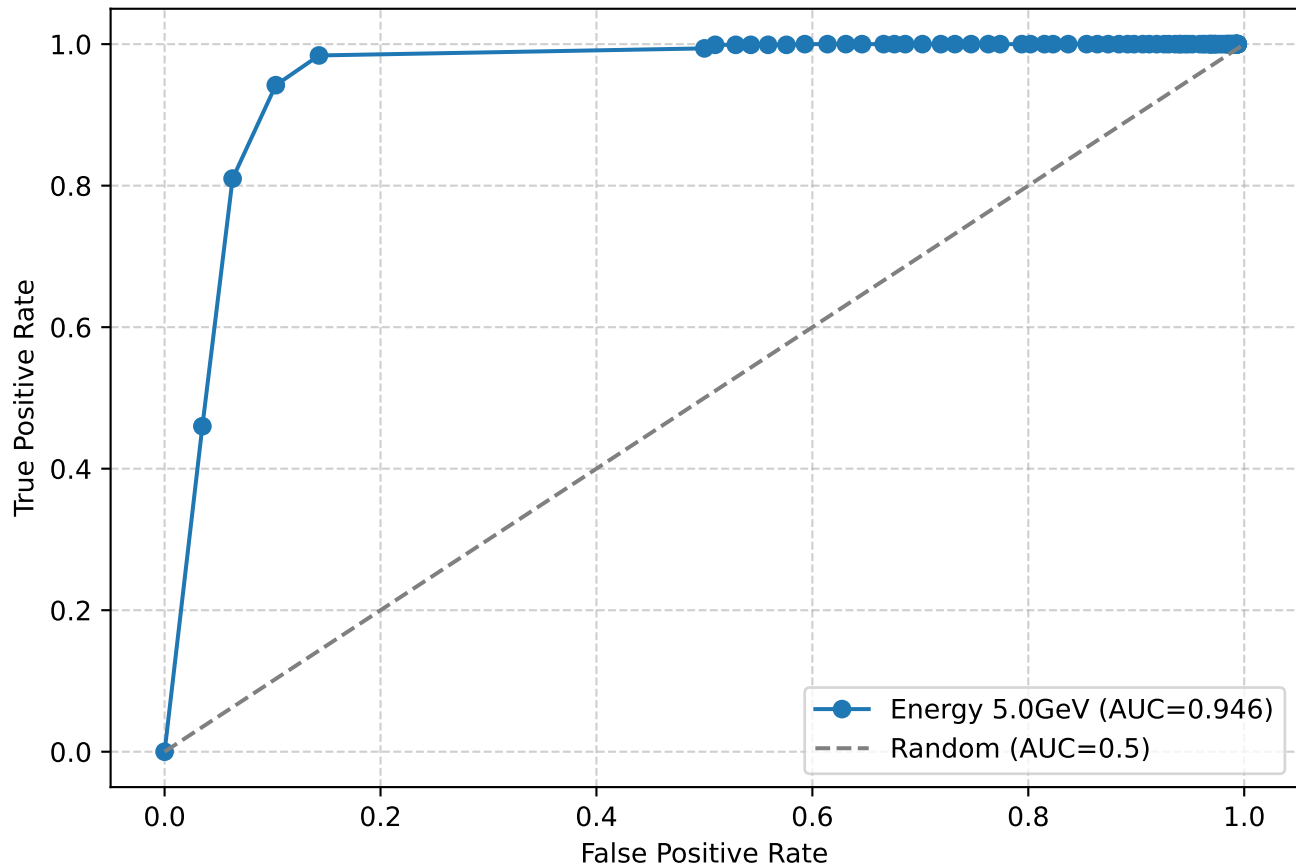
ROC Curve for electrons at 5.0GeV
