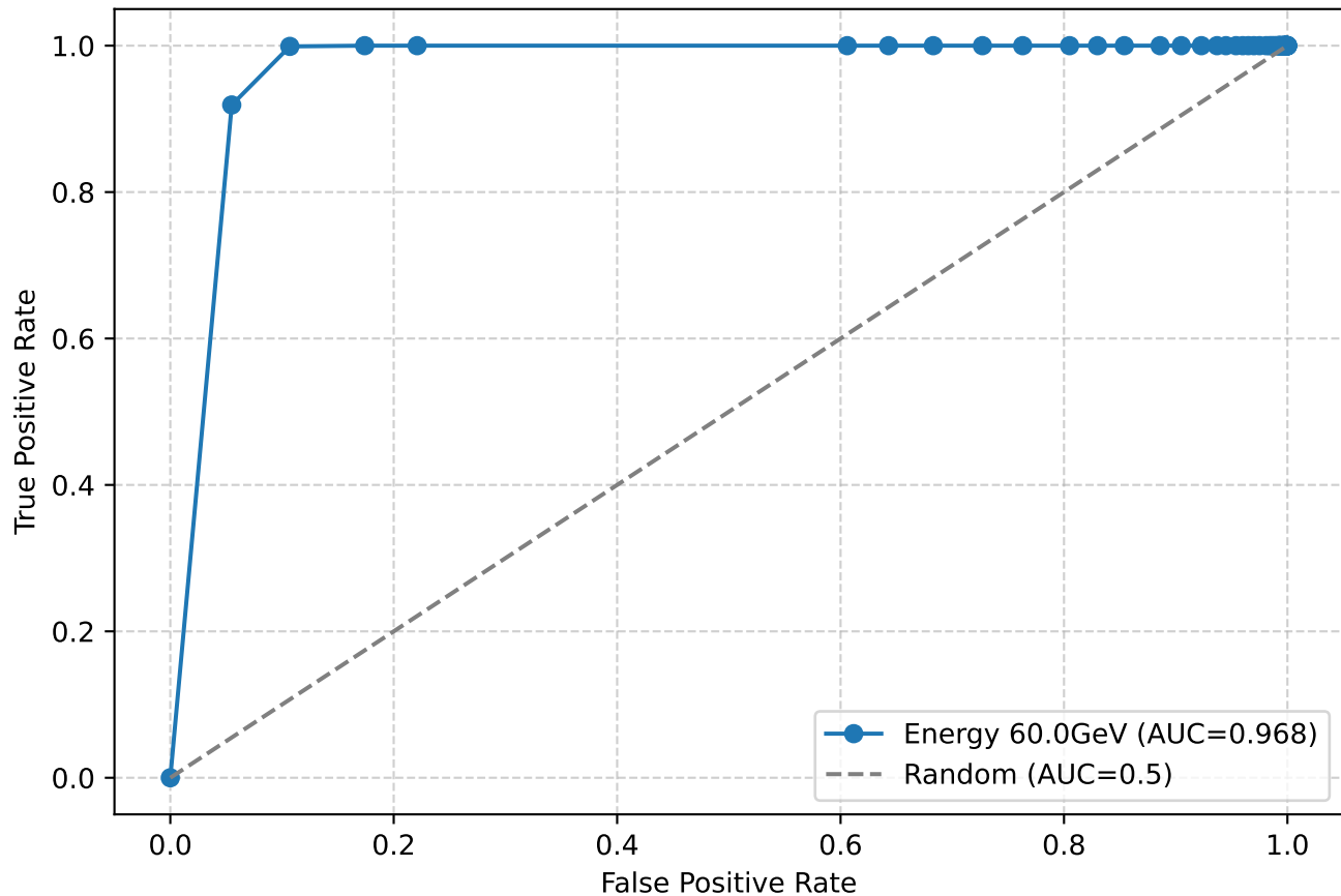
ROC Curve for electrons at 60.0GeV
