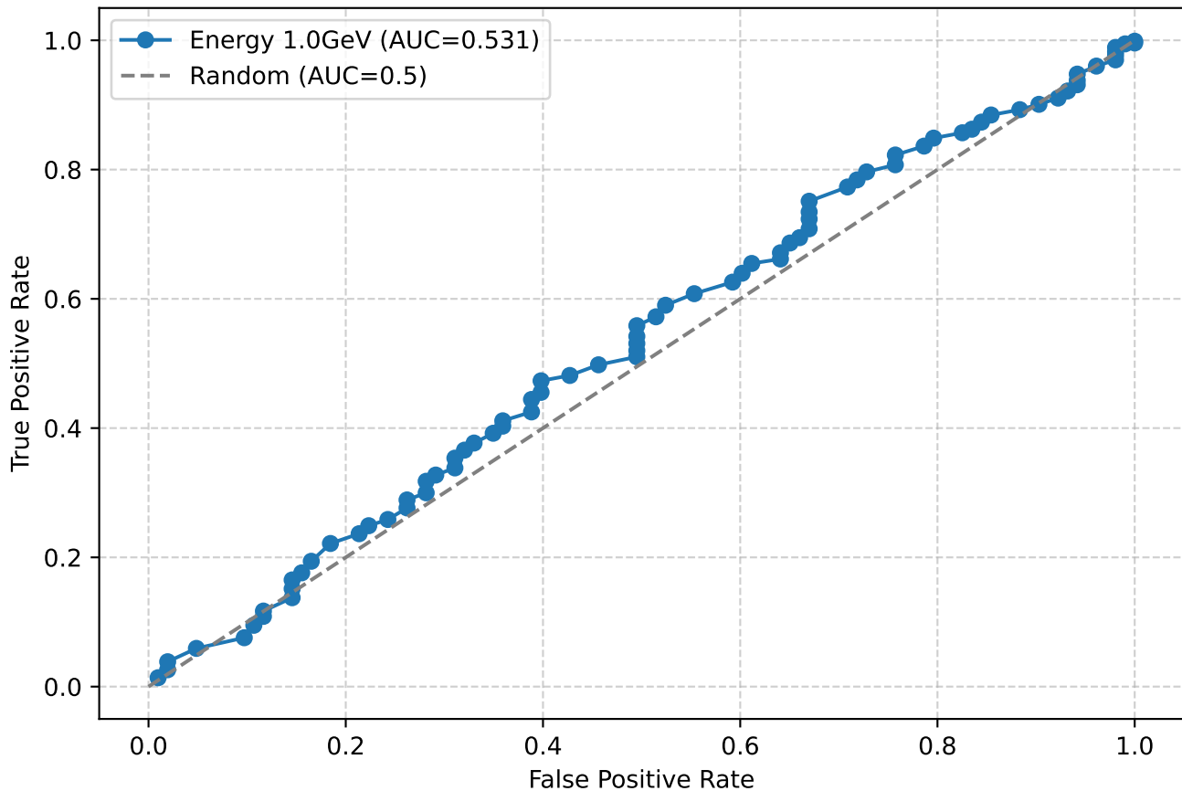
ROC Curve for electrons at 1.0GeV with cuts
