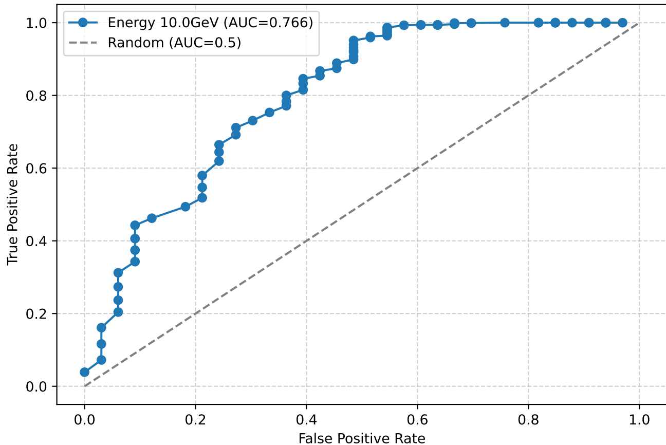
ROC Curve for electrons at 10.0GeV with cuts
