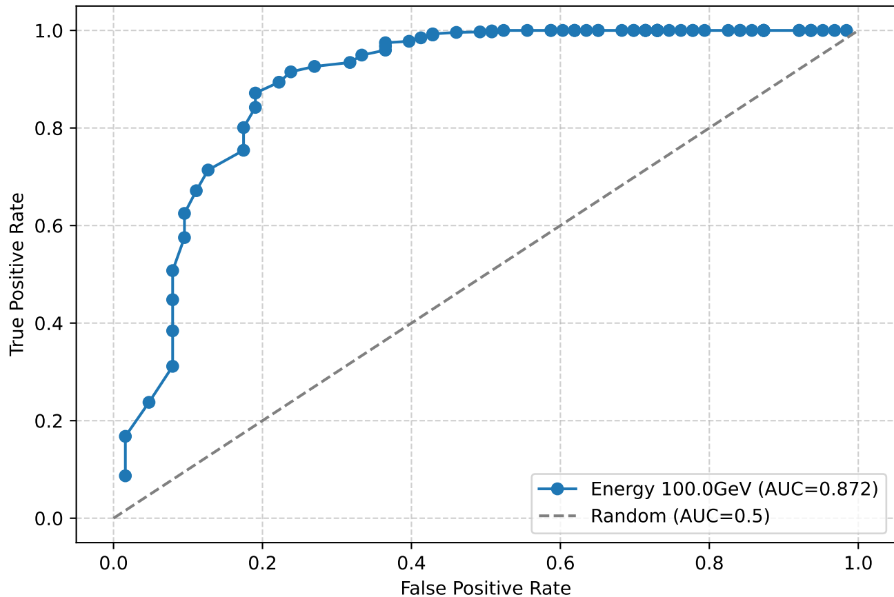
ROC Curve for electrons at 100.0GeV with cuts
