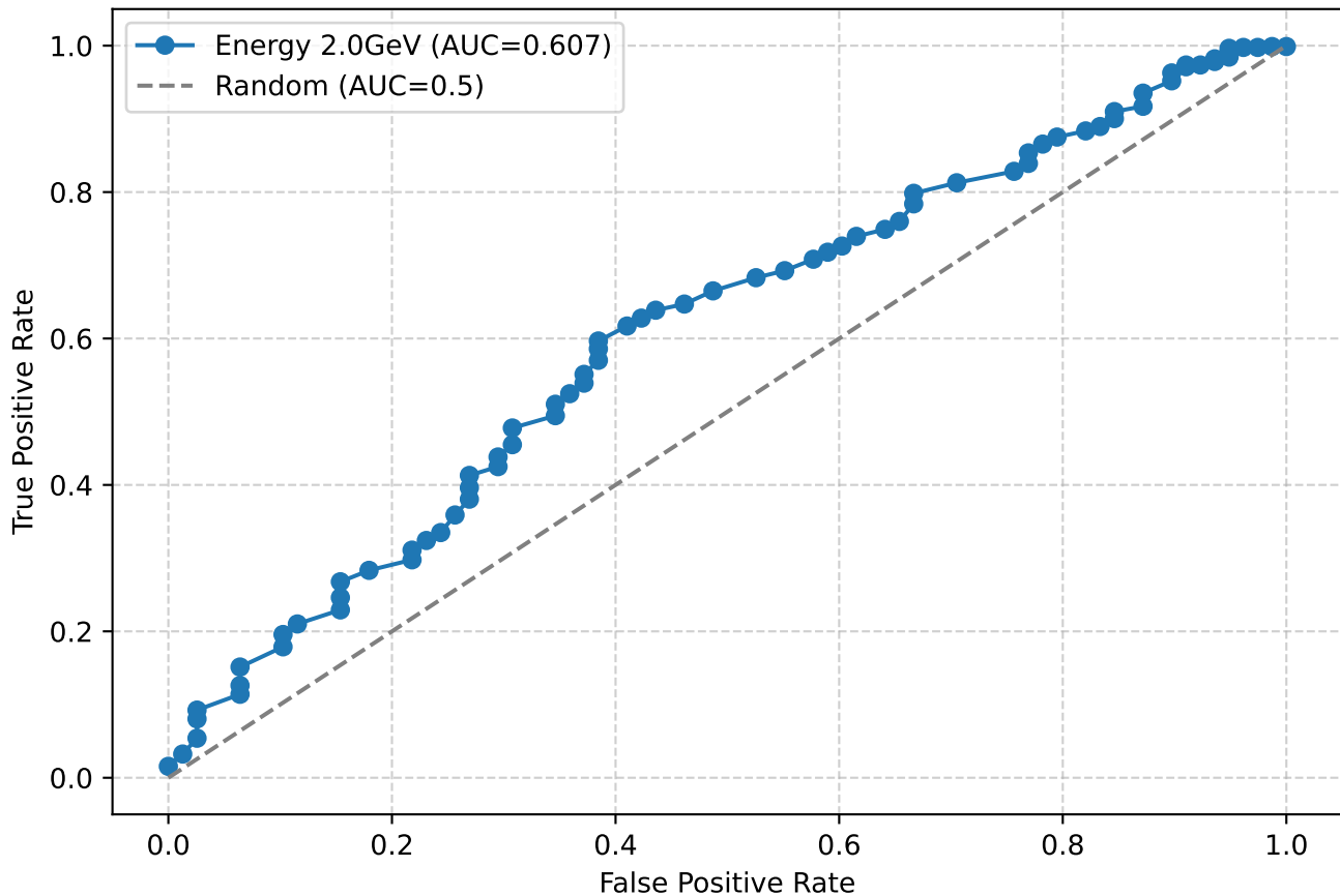
ROC Curve for electrons at 2.0GeV with cuts
