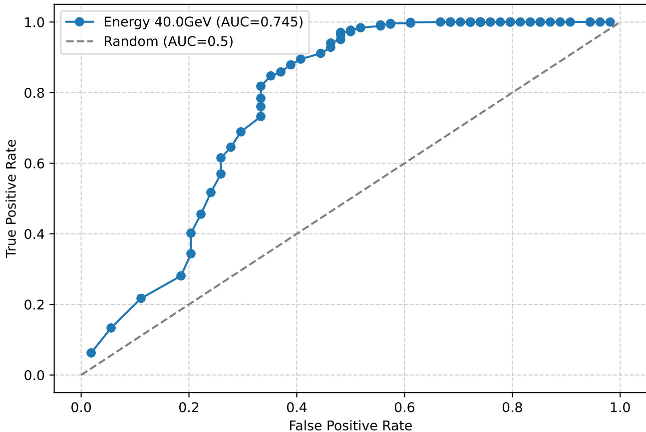
ROC Curve for electrons at 40.0GeV with cuts
