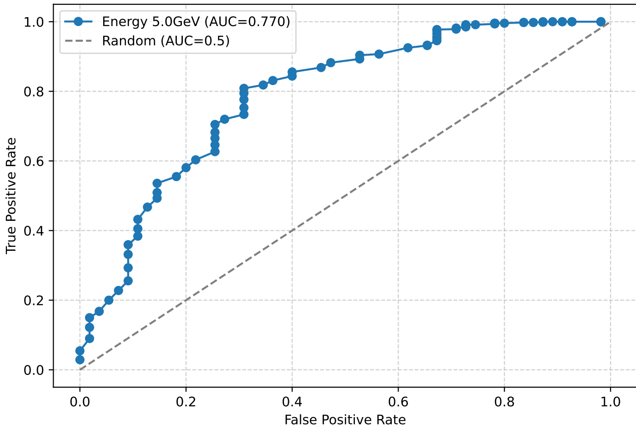
ROC Curve for electrons at 5.0GeV with cuts
