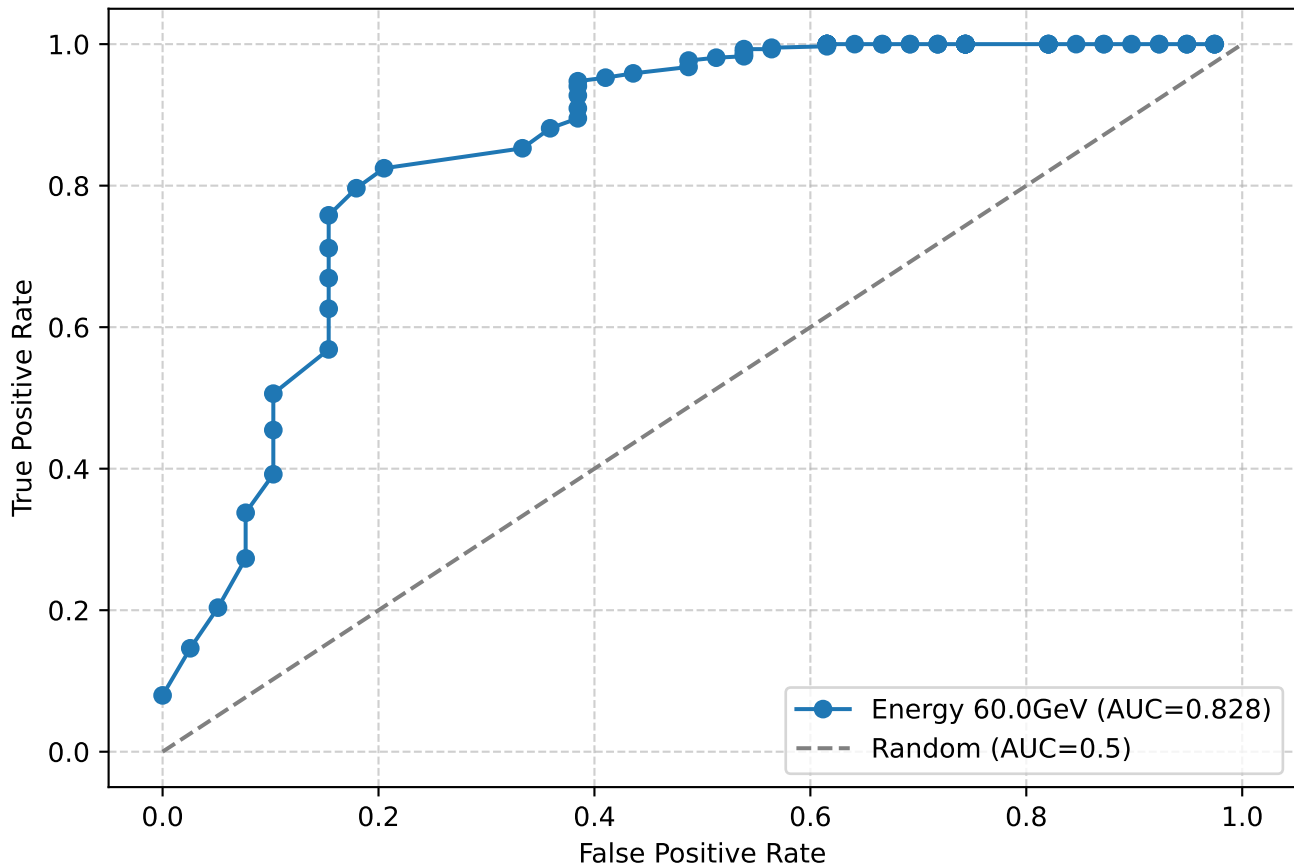
ROC Curve for electrons at 60.0GeV with cuts
