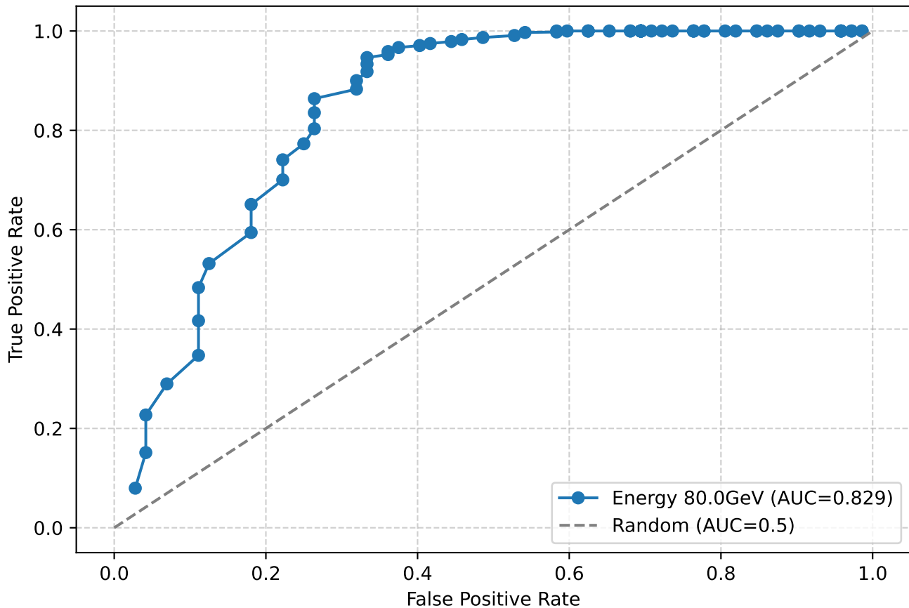
ROC Curve for electrons at 80.0GeV with cuts
