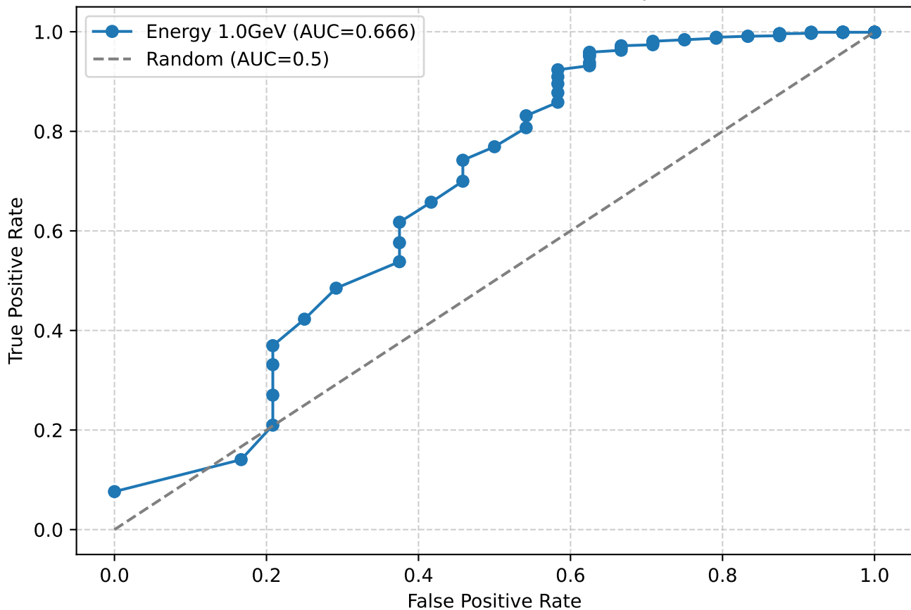
ROC Curve of risetimes for 1.0GeV particles
