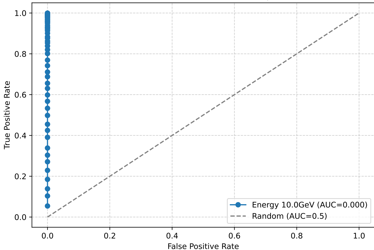
ROC Curve of risetimes for 10.0GeV particles
