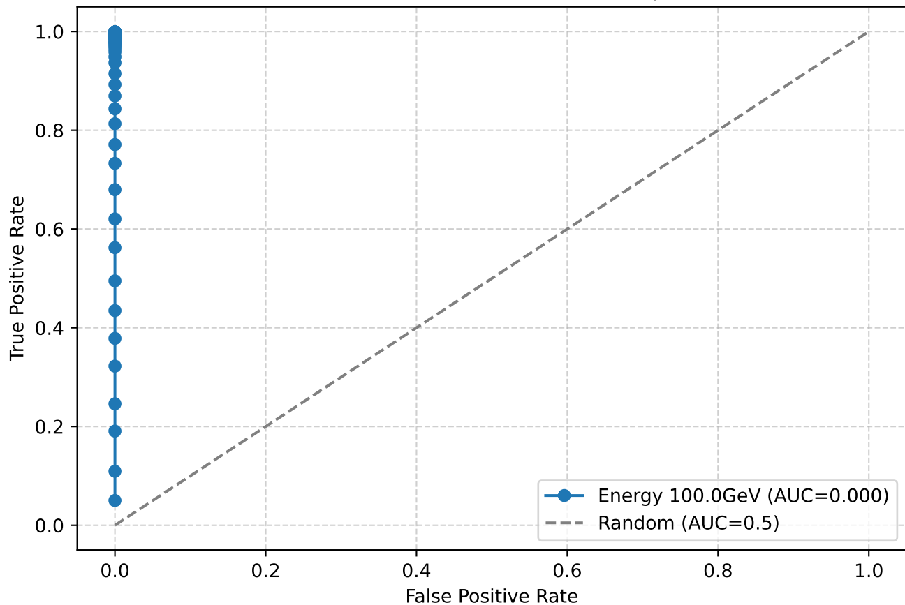
ROC Curve of risetimes for 100.0GeV particles
