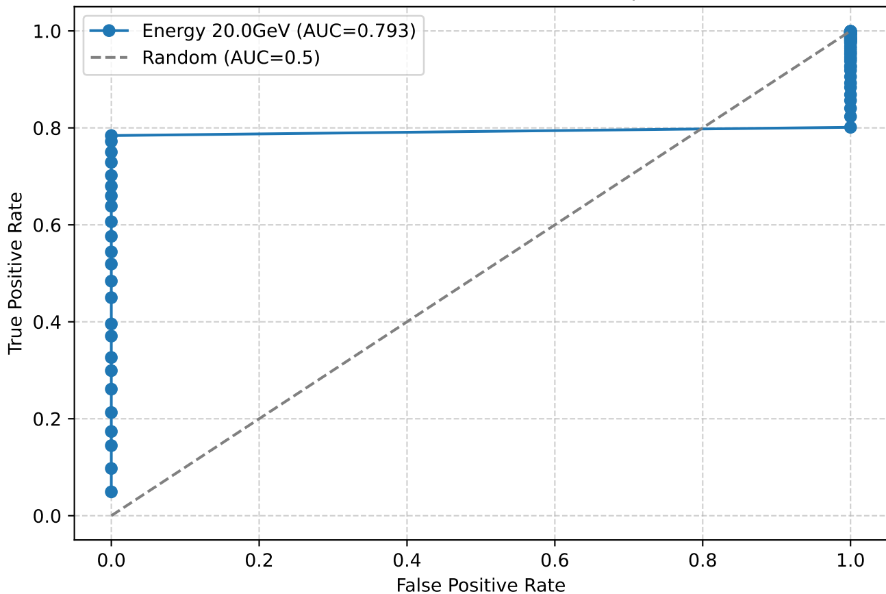
ROC Curve of risetimes for 20.0GeV particles
