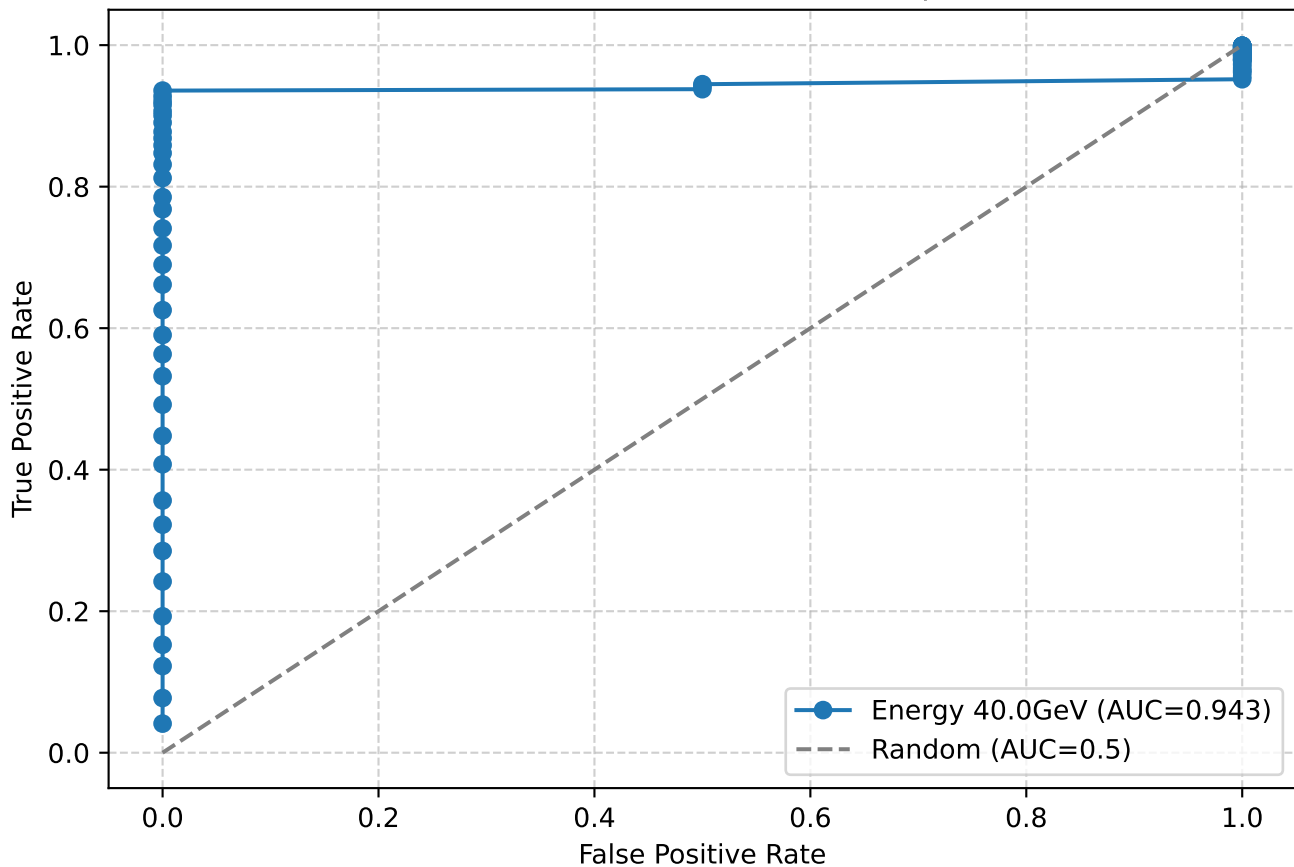
ROC Curve of risetimes for 40.0GeV particles
