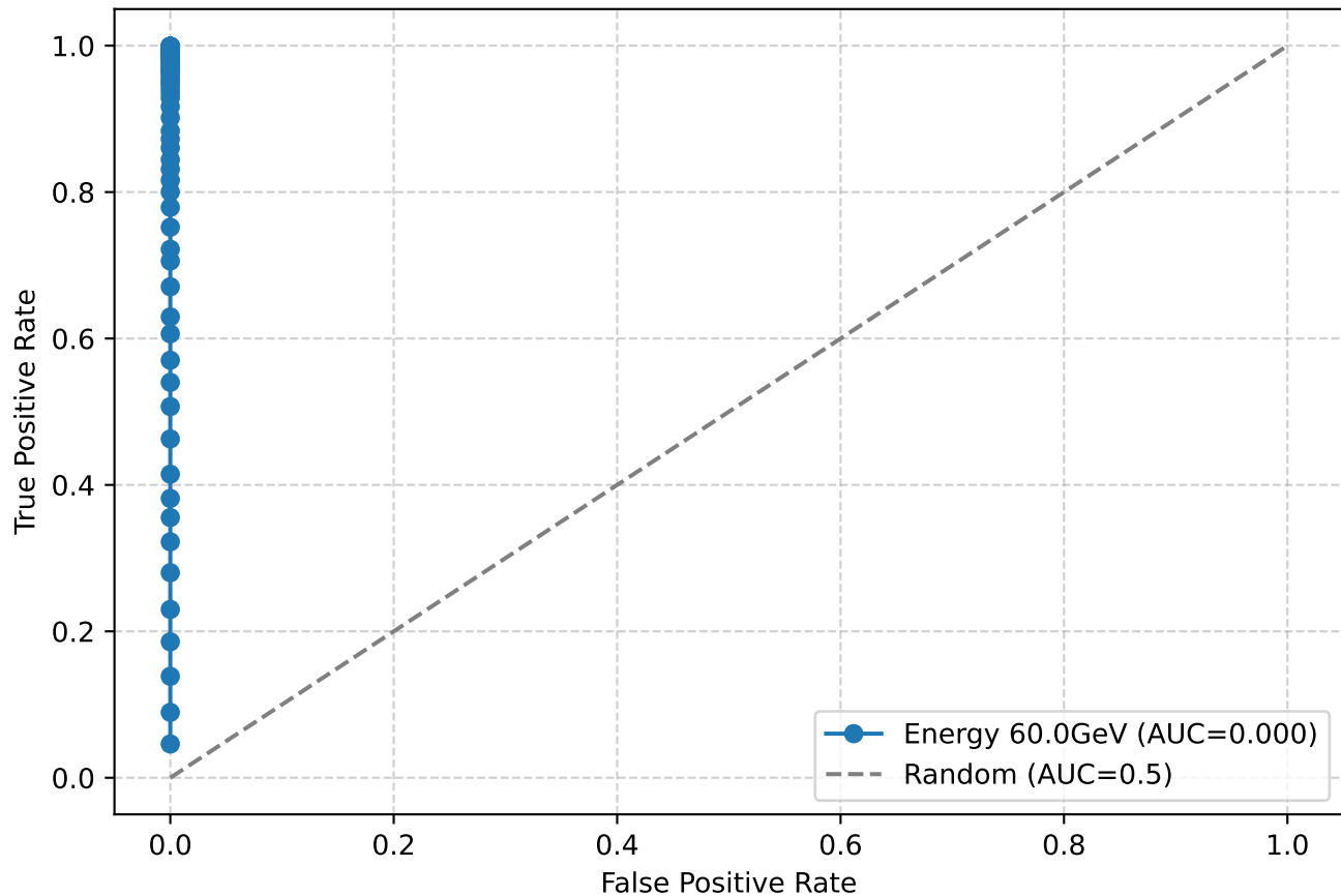
ROC Curve of risetimes for 60.0GeV particles
