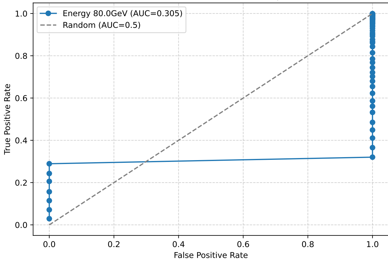
ROC Curve of risetimes for 80.0GeV particles
