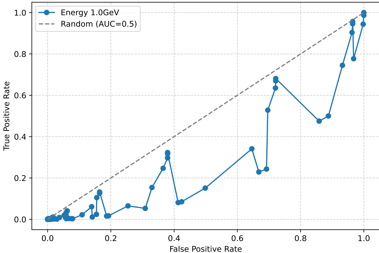
ROC Curve for electrons at 1.0GeV
