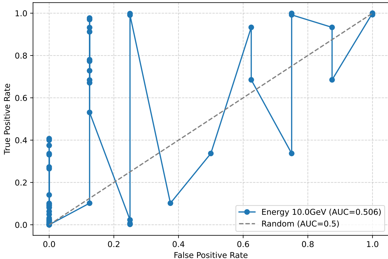
ROC Curve for electrons at 10.0GeV
