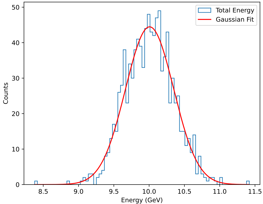
10.0GeV.root: Total Energy
