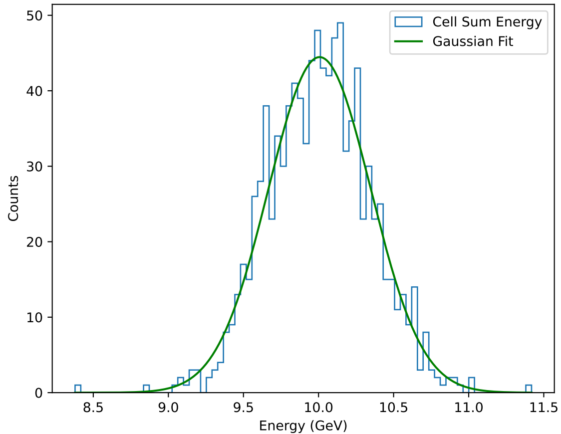
10.0GeV.root: Cell Reconstruction
