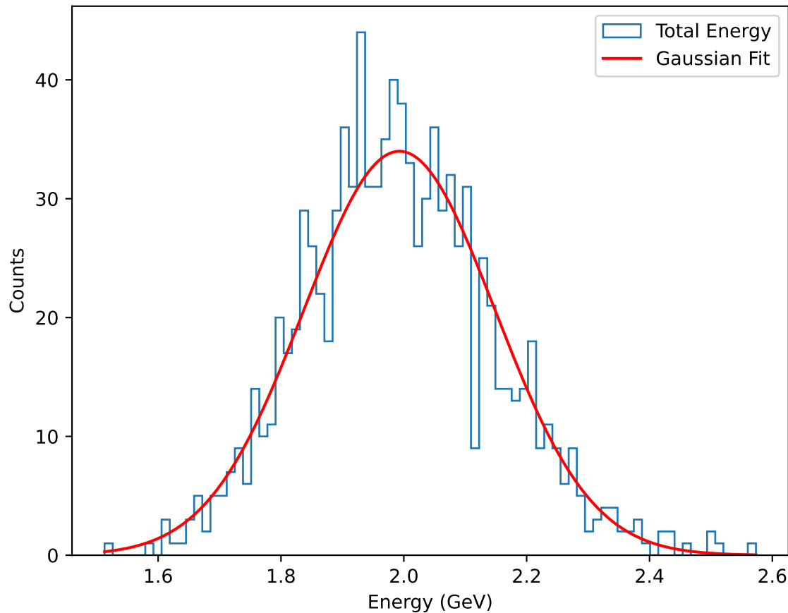
2.0GeV.root: Total Energy
