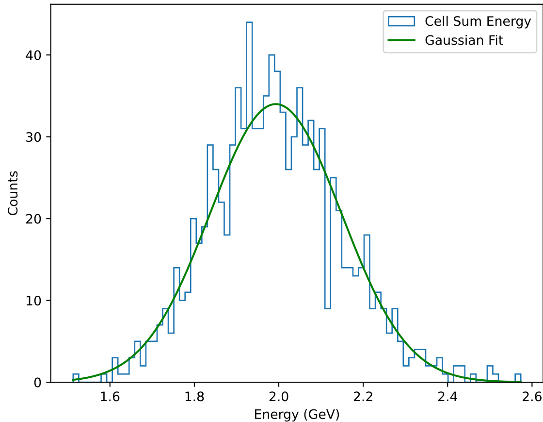
2.0GeV.root: Cell Reconstruction
