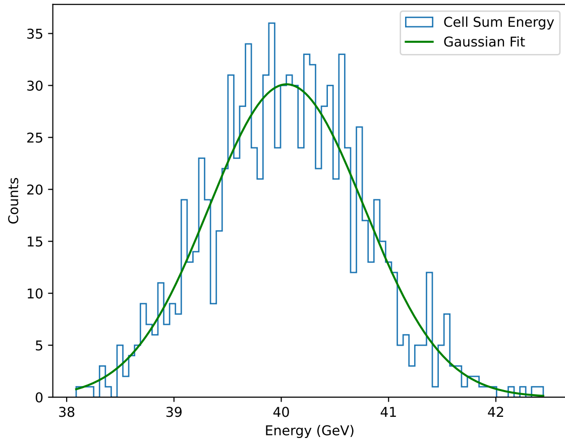
40.0GeV.root: Cell Reconstruction
