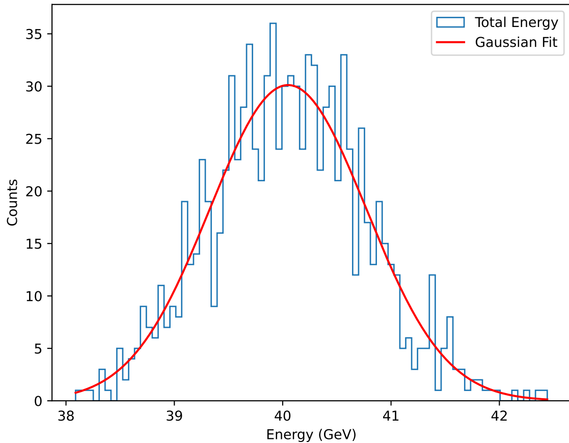
40.0GeV.root: Total Energy
