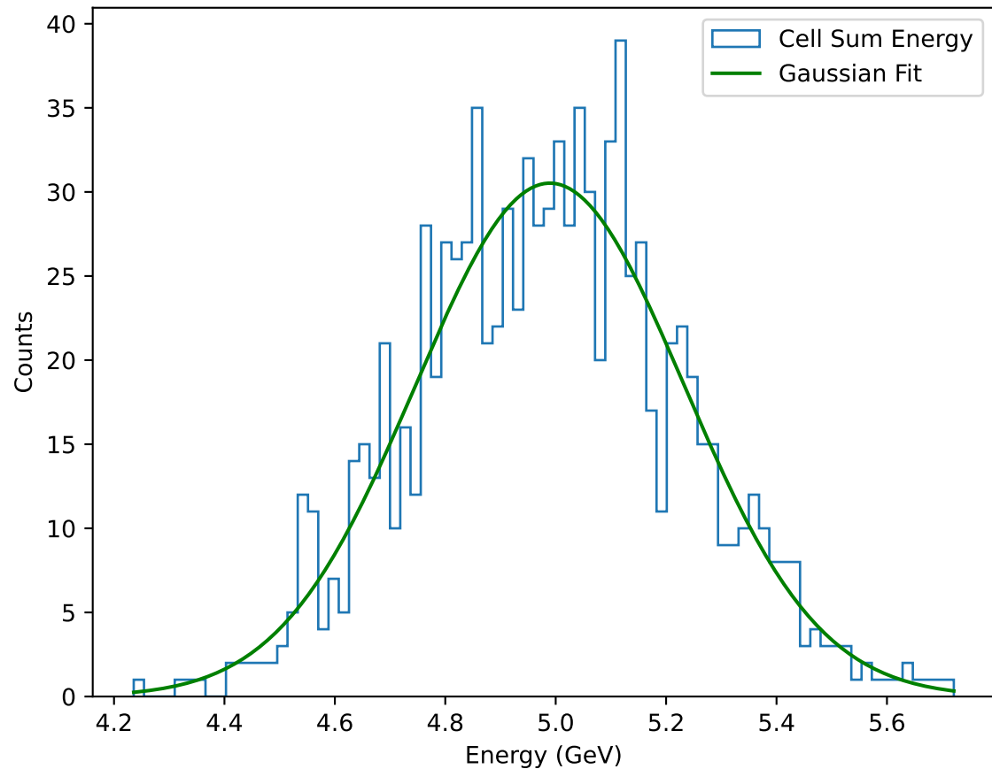
5.0GeV.root: Cell Reconstruction
