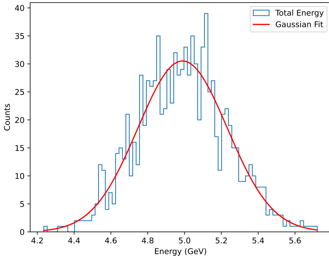
5.0GeV.root: Total Energy
