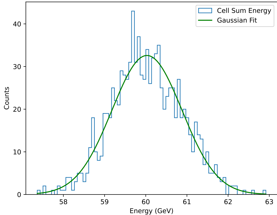
60.0GeV.root: Cell Reconstruction
