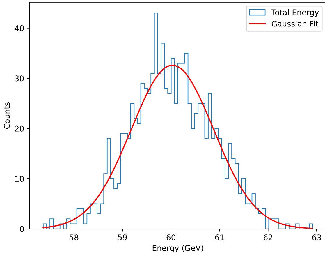
60.0GeV.root: Total Energy
