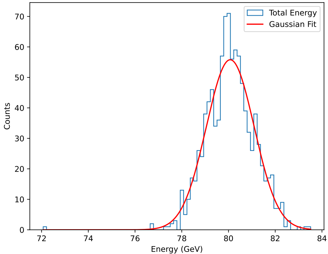
80.0GeV.root: Total Energy
