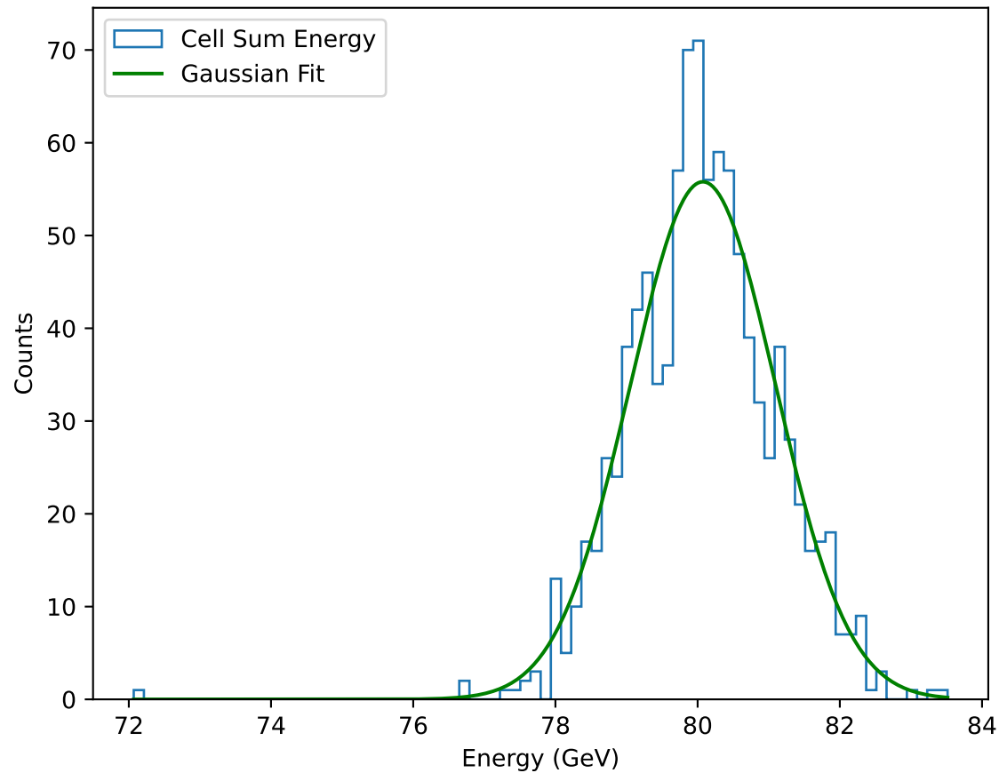
80.0GeV.root: Cell Reconstruction
