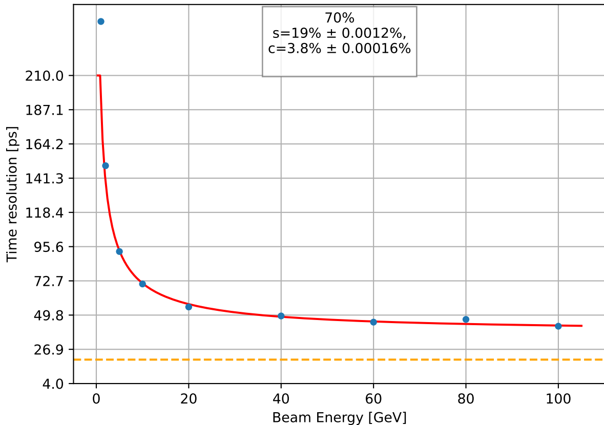
Time Resolution Fit: 70%
