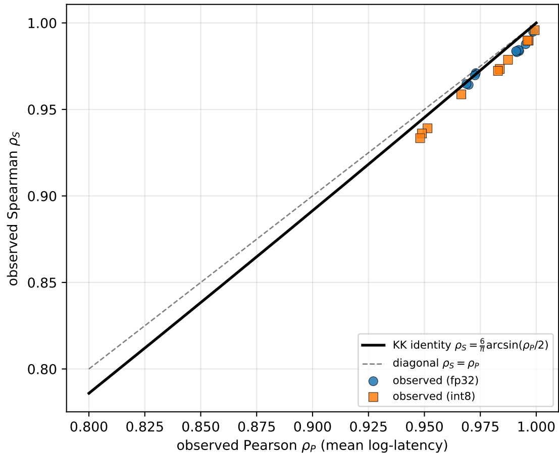
Observed pairs vs Kruskal-Kendall curve (GPU)
