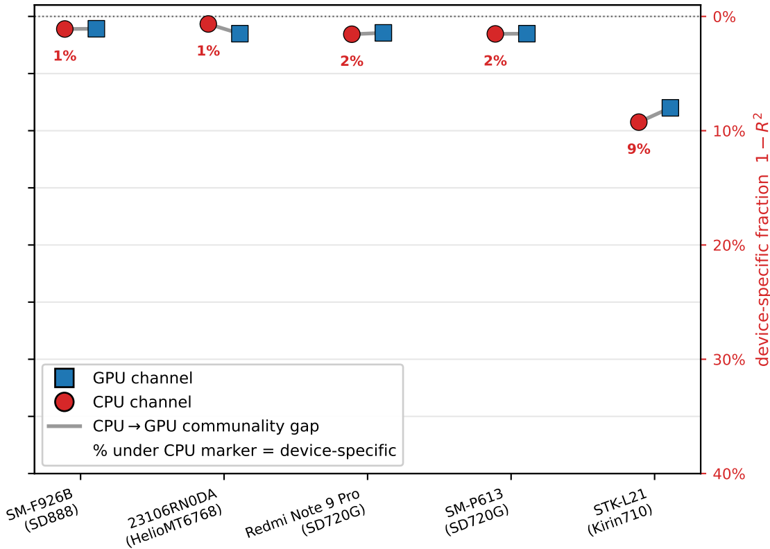
Latent-speed communality R^2_{\text{factor}} — int8
