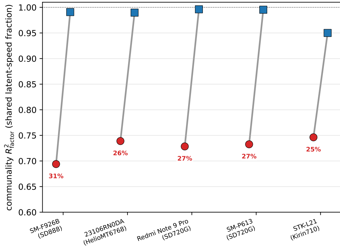
Latent-speed communality R^2_{\text{factor}} — fp32
