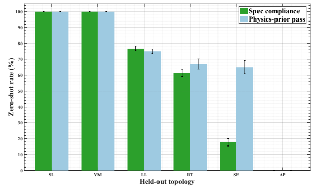
Figure 3: Zero-shot LOOCV per held-out topology (GIN encoder, 3 seeds): full spec compliance (green) and physics-prior pass rate (blue). The gap between the two—widest for Switched Filter—marks designs that are structurally plausible but not yet spec-precise.
