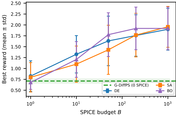
Deployment quality vs. \ per-spec SPICE cost
