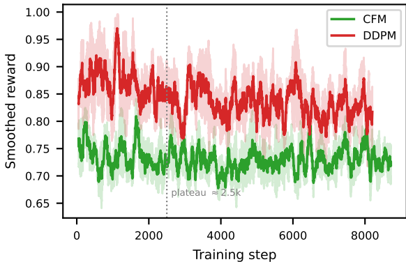
CFM vs. DDPM training dynamics (100-step smooth)
