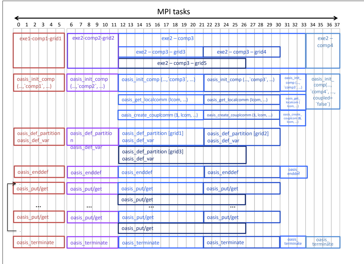
Figure 2.2: The sequence of OASIS3-MCT calls that have to be implemented in the codes so to allow the configuration of components described on figure ???. Each MPI task has to call oasis_init_comp once with the name of its component as 2 nd argument and oasis_terminate before exiting. As none of comp4 tasks is participating to the coupling, comp4 tasks call oasis_init_comp with coupled=.false. as 4 th argument and does not call any other OASIS3-MCT routine except oasis_terminate . As some of comp3 tasks are participating in the coupling, all comp3 tasks have to call oasis_init_comp , oasis_get_localcomm , oasis_create_couplcomm , oasis_enddef and oasis_terminate (these are the only routine to be called by comp3 tasks 31-33 not participating to the coupling). To initialise the coupling exchanges, the tasks of a sub-component holding a field decomposed on a specific grid have to call the oasis_def_partition to express the decomposition of the grid, oasis_def_var to declare the coupling field and oasis_enddef . Finally, the tasks of a sub-component exchanging coupling fields have to call oasis_put and oasis_get accordingly.
