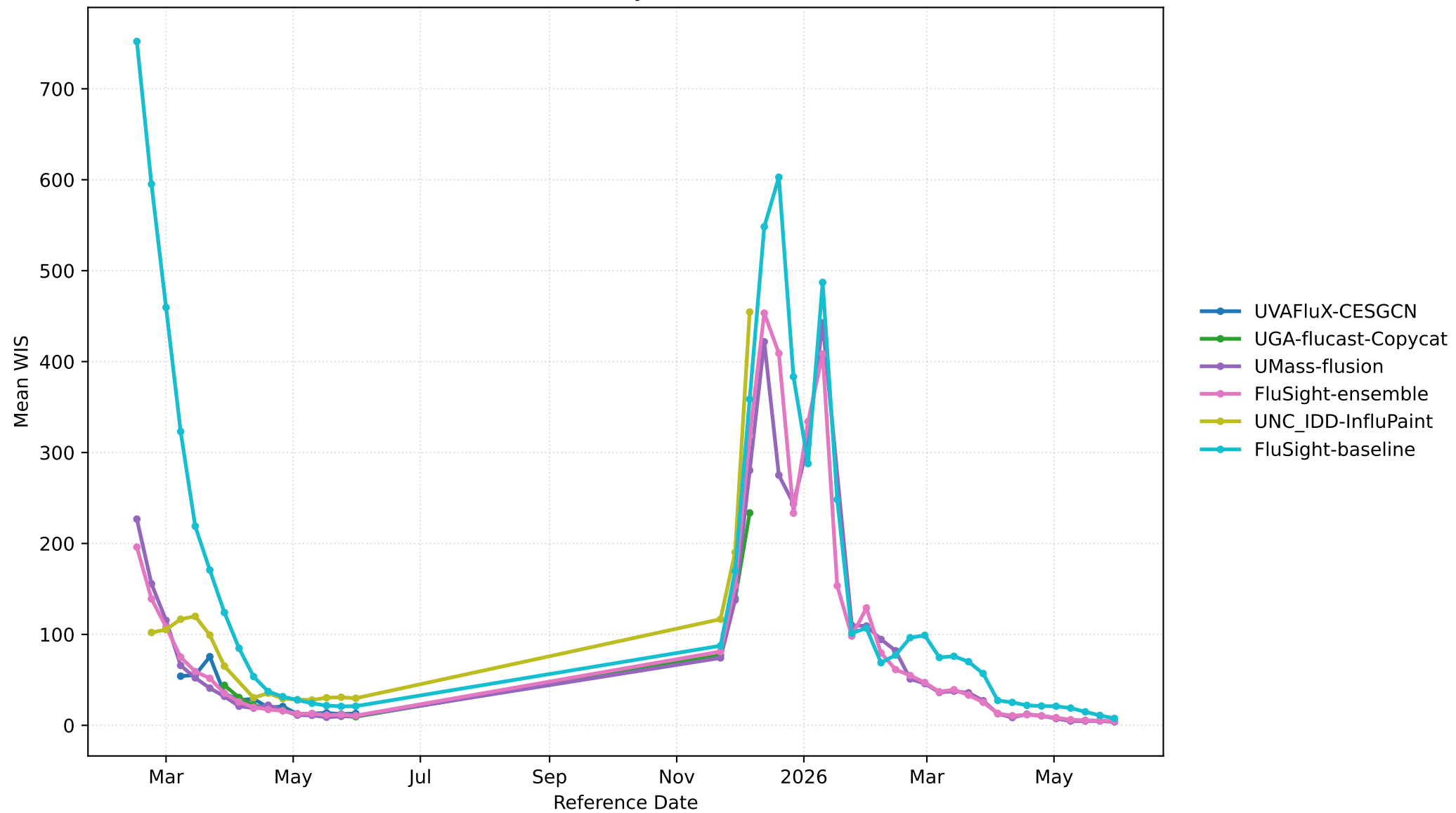
Plot 3. Mean WIS by Reference Date
