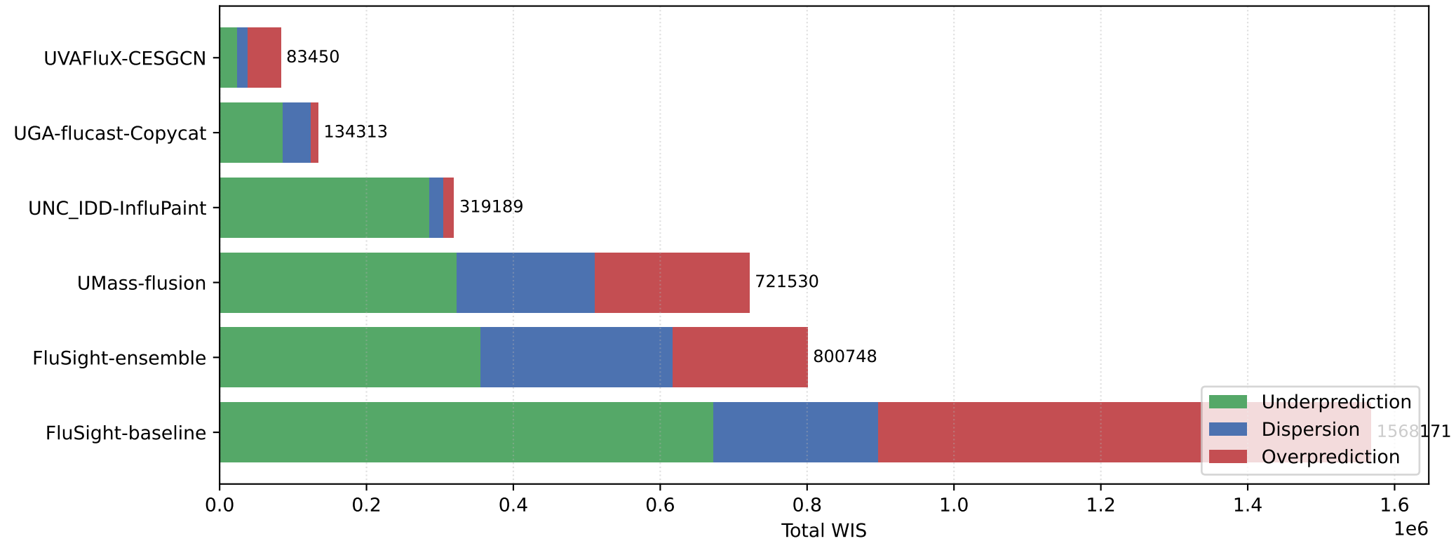
Plot 1. Total WIS Components by Model
