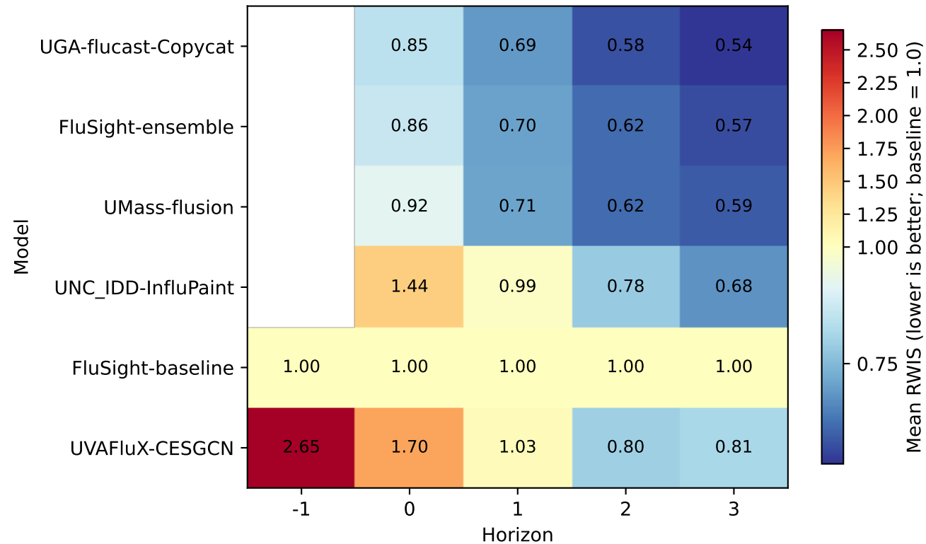
Plot 2. Mean Relative WIS by Model and Horizon
