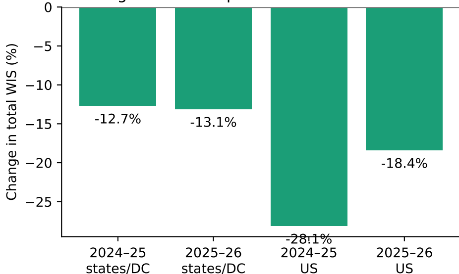
Adding sum WIS improves cumulative forecasts
