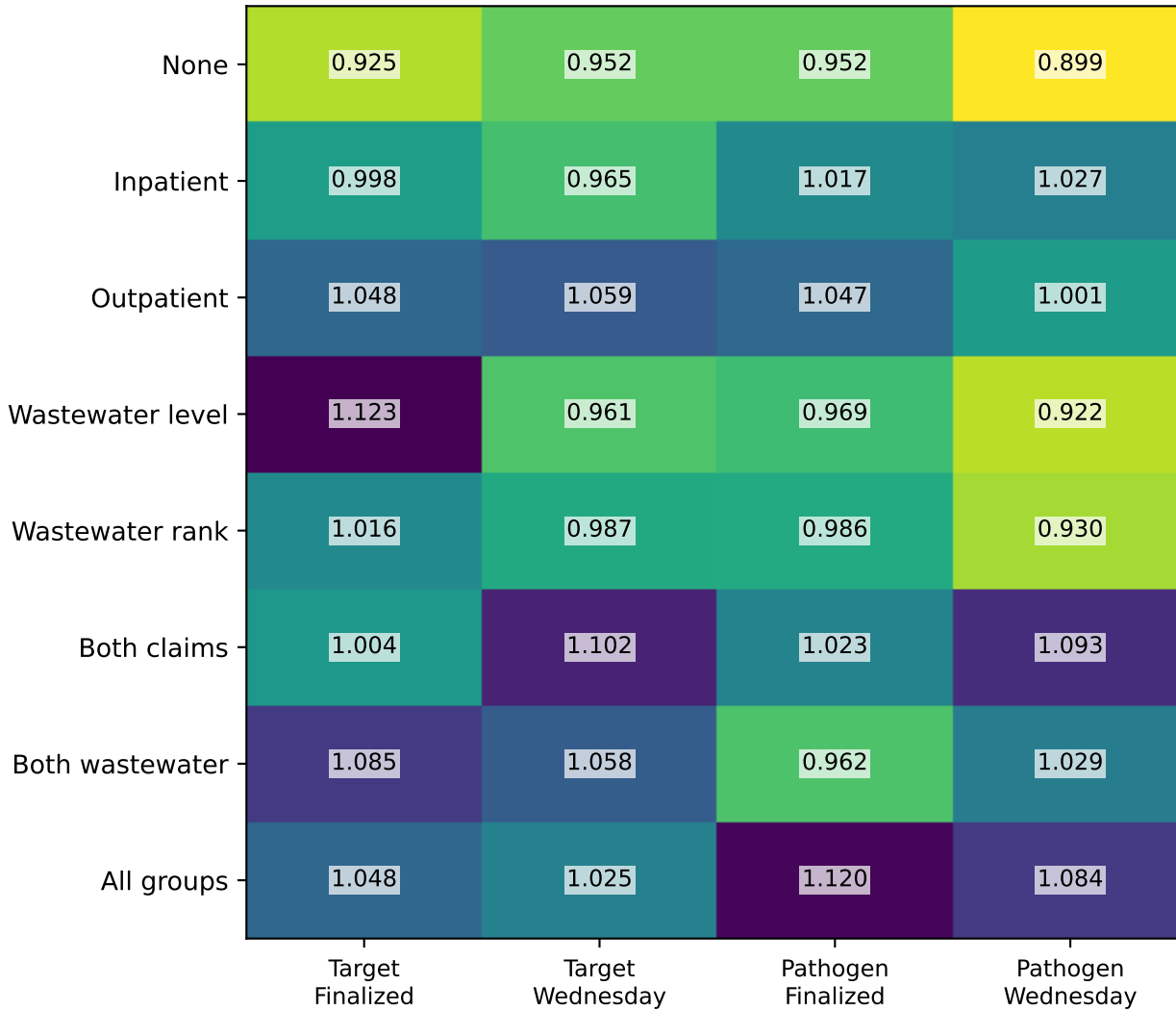
Frozen-Hub relative WIS · lower is better
